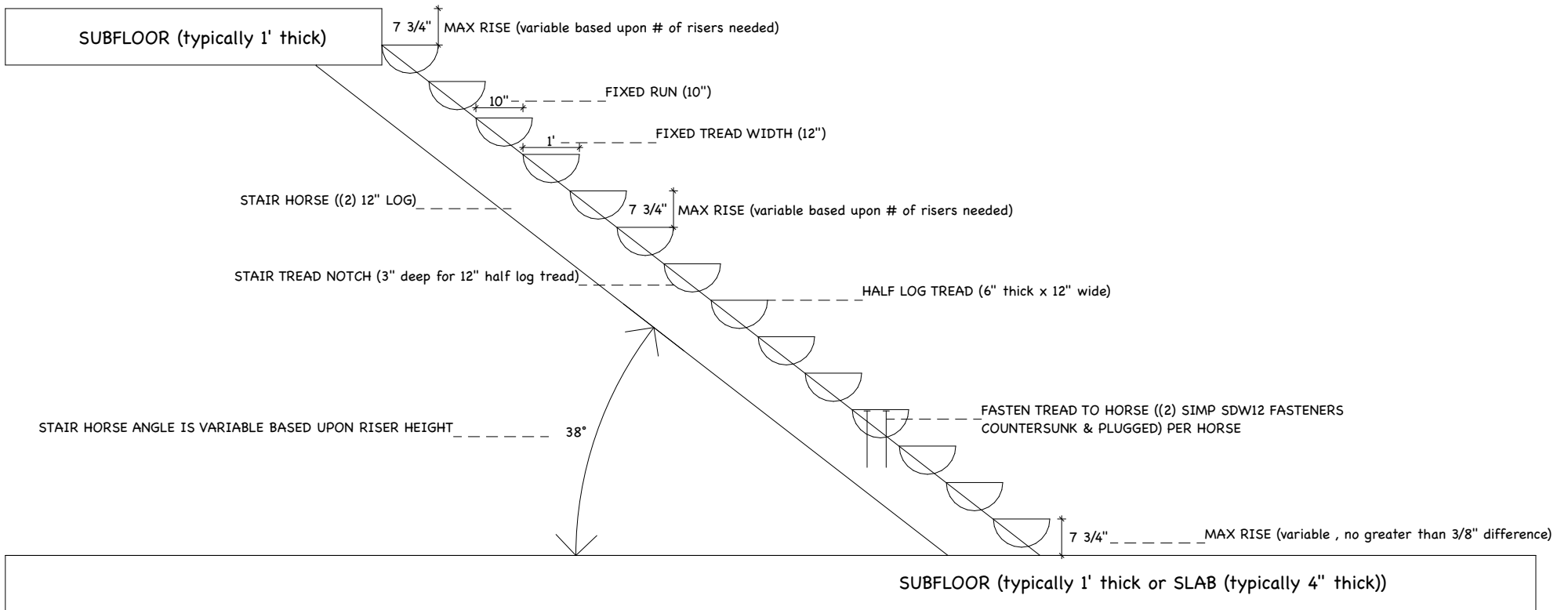
LOG STAIR SYSTEM (12" log horse & treads)
