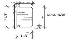
6x8 TIMBER LOG "CHANNEL" STYLE
