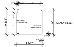
10x10 TIMBER LOG "CHANNEL" STYLE
