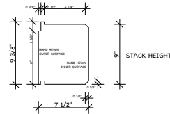
8x10 TIMBER LOG "CHANNEL" STYLE
