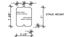
6x8 TIMBER LOG DOUBLE "V" GROOVE
