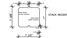
8x8 TIMBER LOG DOUBLE "V" GROOVE
