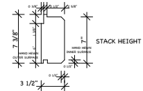
4x8 TIMBER LOG "CHANNEL" STYLE
