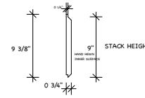
1x10 INTERIOR SIDING "V" STYLE
