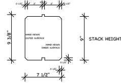
8x10 TIMBER LOG DOUBLE "V" GROOVE
