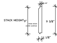
5/4x10 EXTERIOR SIDING "V" STYLE
