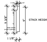
5/4x10 EXTERIOR SIDING "CHANNEL" STYLE
