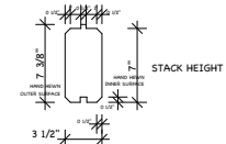
4x8 TIMBER LOG DOUBLE "V" GROOVE
