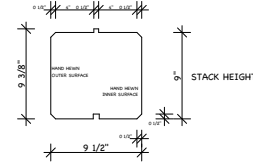
10x10 TIMBER LOG DOUBLE "V" GROOVE
