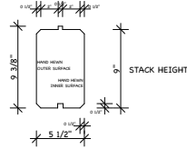
6x10 TIMBER LOG DOUBLE "V" GROOVE
