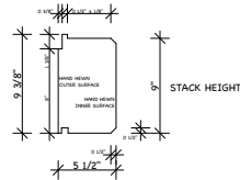
6x10 TIMBER LOG "CHANNEL" STYLE
