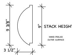
10" ROUND LOG SIDING 4x10 SHIP LAP
