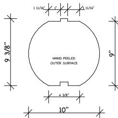
10" ROUND LOG TONGUE & GROOVE
