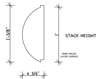
13" ROUND LOG SIDING 5x13 SHIP LAP
