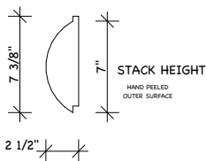
8" ROUND LOG SIDING 3x8 SHIP LAP
