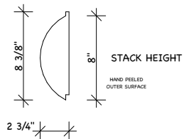
9" ROUND LOG SIDING 3x9 SHIP LAP
