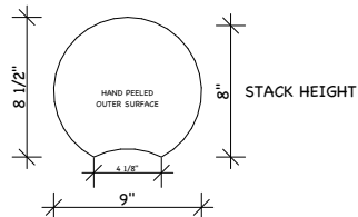
9" ROUND LOG SWEDISH COPE
