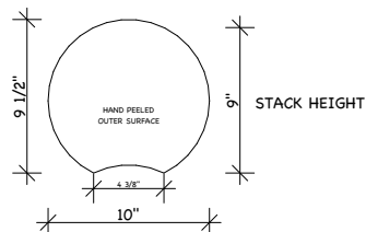
10" ROUND LOG SWEDISH COPE
