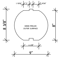
9" ROUND LOG TONGUE & GROOVE
