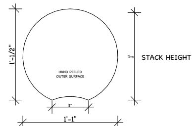
13" ROUND LOG SWEDISH COPE
