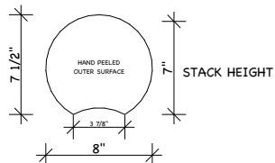
8" ROUND LOG SWEDISH COPE
