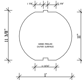
12" ROUND LOG TONGUE & GROOVE
