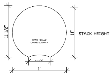
12" ROUND LOG SWEDISH COPE
