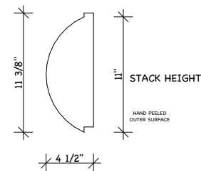
12" ROUND LOG SIDING 5x12 SHIP LAP
