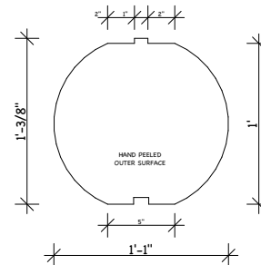
13" ROUND LOG TONGUE & GROOVE
