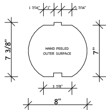
8" ROUND LOG TONGUE & GROOVE
