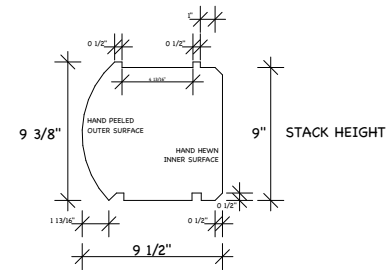
10x10 JUMBO D LOG
