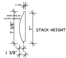
2x8 D LOG SIDING
