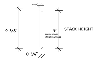
1x10 INTERIOR SIDING "V" GROOVE STYLE
