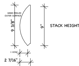
3x10 JUMBO D LOG SIDING
