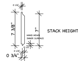
1x8 INTERIOR SIDING "V" GROOVE STYLE
