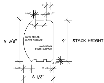
7x10 JUMBO D LOG
